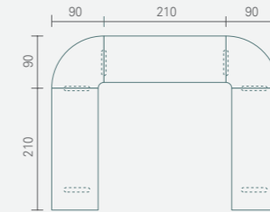
MX1639 L390 P300 H75
