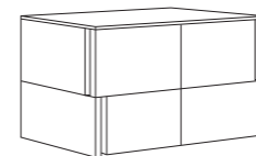
comò 4 cassettoni chest of drawers with 4 big drawers cm. L. 136,2 x P. 56,4 x H. 71
